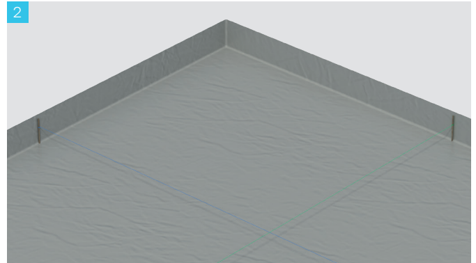
2 Measure the distances to the walls and edges. Set up the string line following the joint location.
