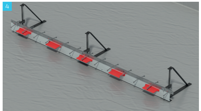
4 Fit ArmourJacks to the ArmourJoint top strips.
