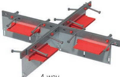
4-way Intersection
